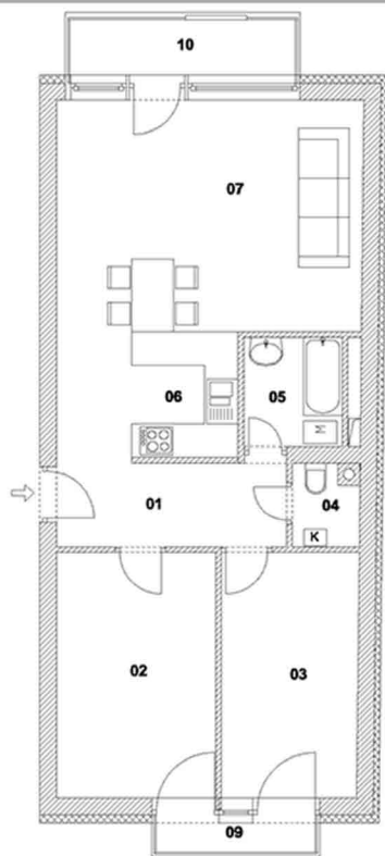
II. EMELET "A" 2/5 LAKÁS
